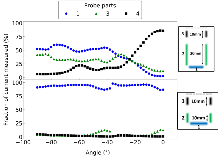
Figure 5.23: Fraction of current measured by electrode 1 (blue), 2 (red), 3 (green) and 4 (black). The probe is composed of staged electrodes as displayed by the picture on the right. Each electrode is spaced by a 10 mm long PEEK insulator. The values are relative to the total current measured by all electrodes. HT2 fires at 0.66 A and 250 V.
