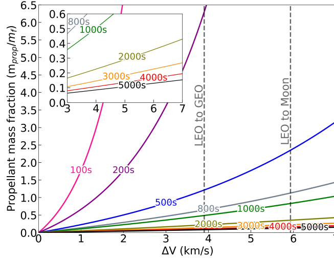
Figure 1.1: Evolution of the propellant mass to the spacecraft dry mass fraction against typical \Delta V values given for different Isp. The dashed lines represents \Delta V manoeuvres from low Earth orbit (LEO) to geostationary orbit (GEO) or to the Moon.
