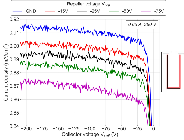
Figure 5.3: I-V curves acquired for different repeller voltages at 0^\circ with configuration 50.A1.05.P - F.A1.4. HT1 fires at 250 V and 0.66 A.
