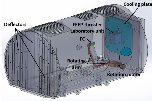
Figure 3.2: 3-D model of the FEPP experimental apparatus in the FH chamber.
