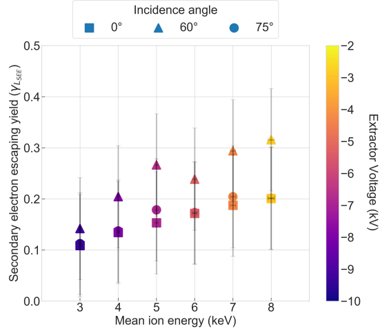
Figure 4.21: Ion-induced electron escaping yield obtained with the ion source LU-C for different collector geometries. The thruster fires in at 2 mA.
