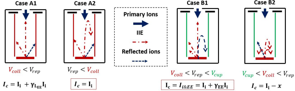
Figure 4.4: Explanation of the measurement method to obtain \gamma_{EE}
