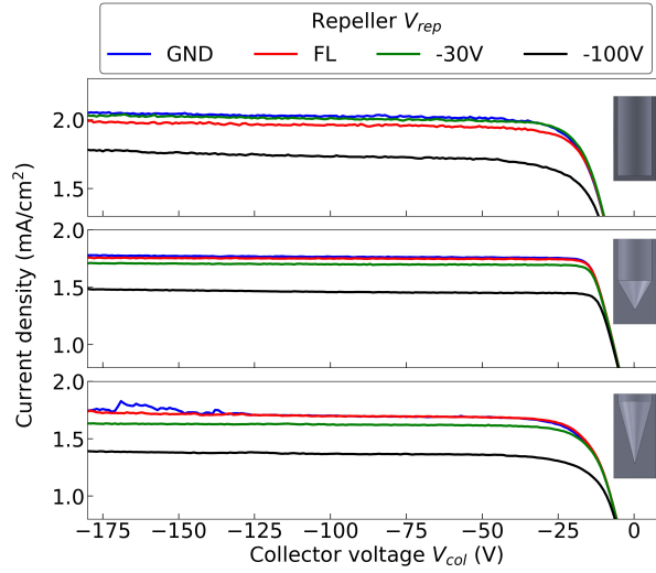
Figure 5.15: I-V curved acquired at 0^\circ with different cup shape: flat (top), conical with 60^\circ (middle) and conical with 30^\circ (bottom). The repeller is set to grounded, floating, -30 V and -100 V. HT2 fires at 0.66 A and 300 V.
