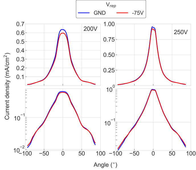
Figure 5.2: Current density angular profile acquired with FC 50.A1.05. P - F.A1.4 with the repeller grounded or biased to -75 V. HT1 fires at 0.66 A, 200 V (left) and 250 V (right). Profiles are displayed with a linear (top) and logarithmic (bottom) scale.
