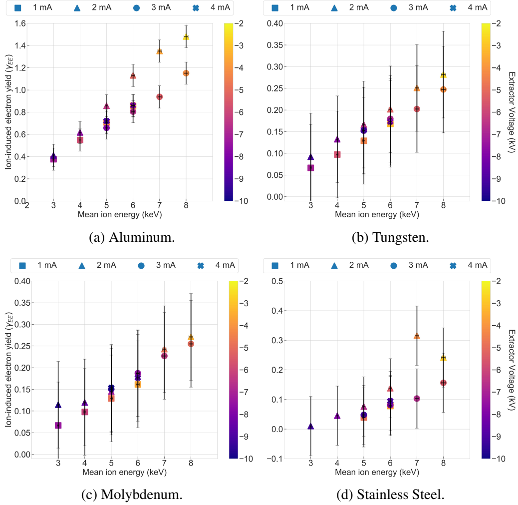
Figure 4.8: Ion-induced electron yield ( \gamma_{EE} ) from different flat ion collector obtained with the thruster LU-C firing at 1, 2, 3 and 4 mA. The ion bombardment is normal to the target.
