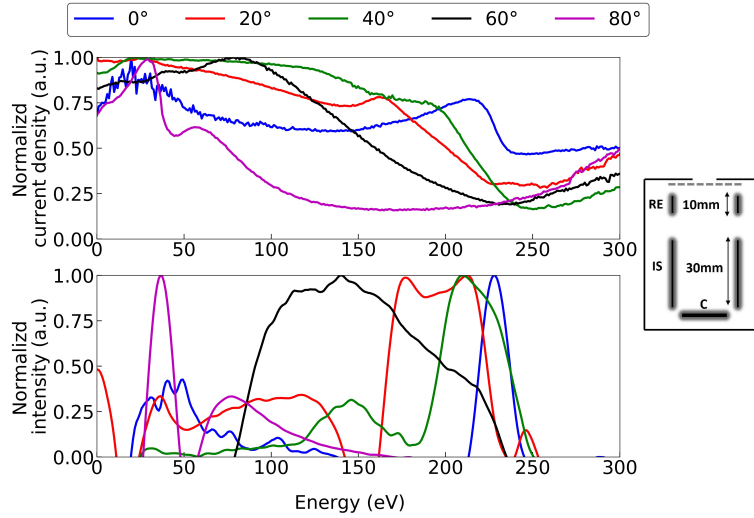
Figure 6.20: Ion current density and normalized energy distribution acquired with the DMP configured as an energy analyser. RE is 10 mm, IS is 30 mm and C is made of molybdenum. HT2 fires at 0.66 A and 250 V. The probe scan the ion energy at different angular positions from 0^\circ to 80^\circ .
