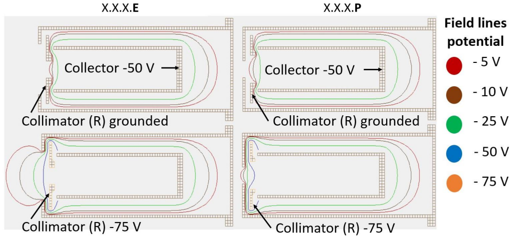
Figure 5.1: Field lines computed with SIMION. Configurations X.X.X.E (left) and X.X.X.P (right) with the repeller grounded (top) and at -75 V (bottom).
