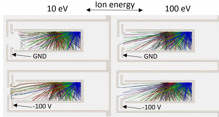
Figure 5.7: Ion simulations performed with the software SIMION. Each configuration displays the possible trajectory of ion rebounds from the lateral side of the FC. The colour refers to different rebound location. The collector is at -50 V. The repeller is either grounded (top) or biased to -100 V (bottom). Ion energies are 10 eV (left) and 100 eV (right).
