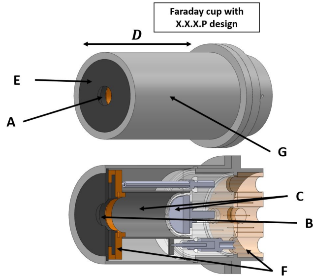
Figure 6.23: Drawing of a Faraday cup design suitable to study the plume of a FEED, low power RIT and low power Hall thruster. A = Probe aperture, B = Repeller aperture, C = Collector, D = Collector cup length, E = Front material, F = Insulators, G = Housing
