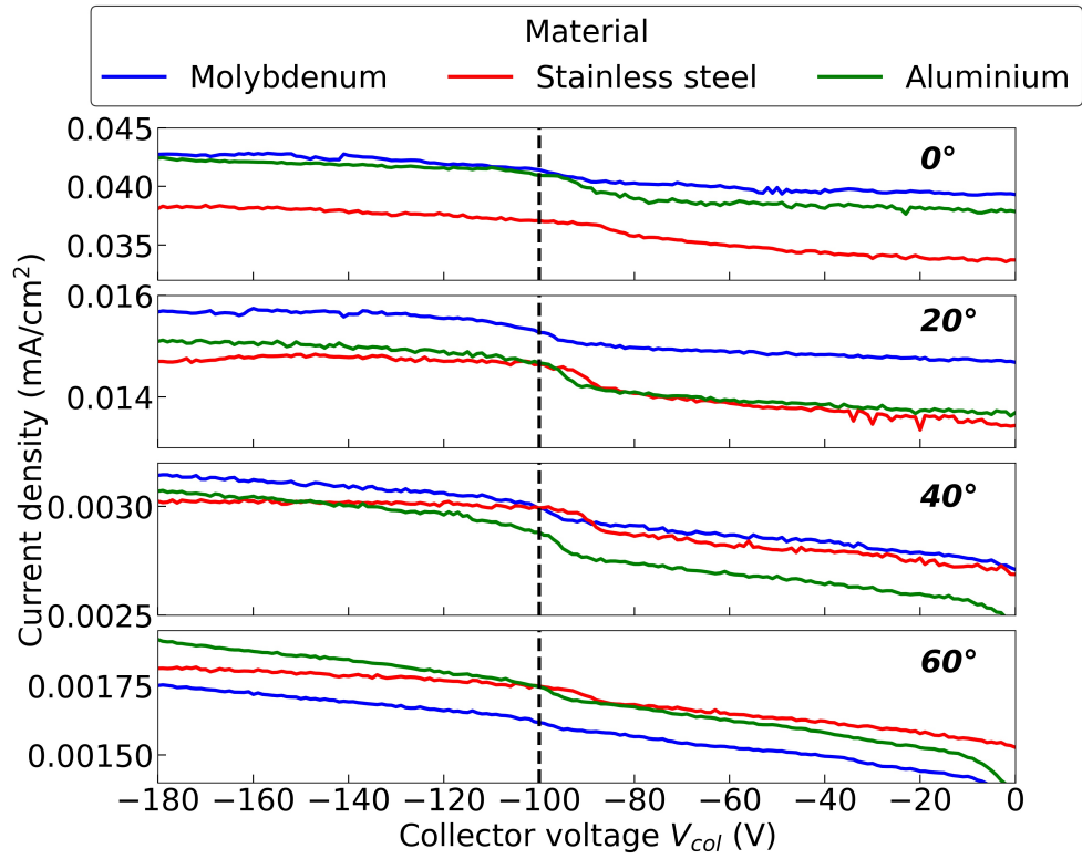
Figure 5.9: I-V curves acquired with 12 mm disks made of molybdenum (blue), stainless steel (red) and aluminium (green). The grid placed upstream the disk is biased to -100 V. HT2 fires at 0.66 A and 300 V.
