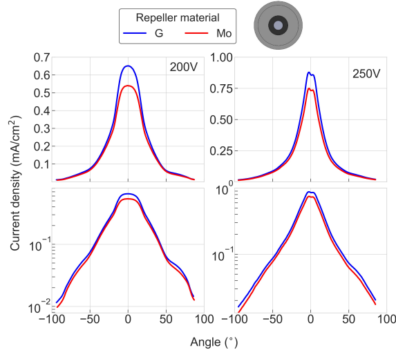
Figure 5.24: Ion current density angular distribution acquired with FC 50. G .10.E - F.A1.4 (blue) and 50. Mo .10.E - F.A1.4 (red). HT1 fires at 0.66 A, 200 V (left) and 250 V (right). Profiles are displayed with a linear (top) and logarithmic (bottom) scale.
