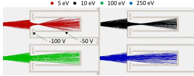
Figure 5.5: Ion simulations performed with the software SIMION. Each configuration displays the ion trajectory going through the FC. Potential is fixed at -50 V and -100 V for the collector and repeller, respectively. Ion energies are 5 eV (red), 10 eV (black), 100 eV (green) and 250 eV (blue). The probe aperture diameter is 5 mm.
