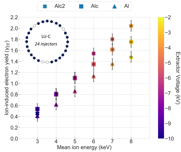
Figure 4.11: Ion-induced electron yield obtained with the ion source LU-C for different collector geometries. The thruster fires in mode 2.
