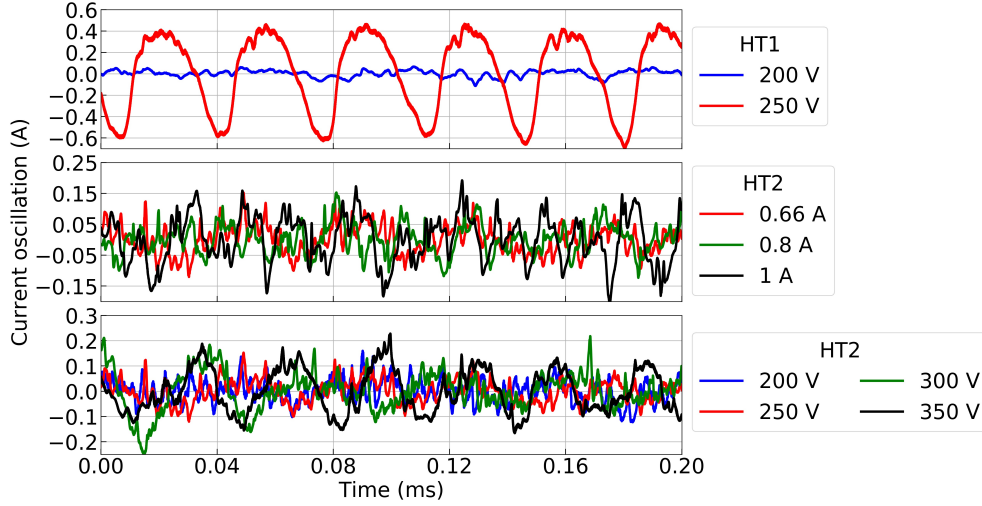
Figure 3.12: Discharge current oscillations for HT1 and HT2. Top: HT1 firing at 0.66 A, 200 V and 250 V. Middle: HT2 in operation at 0.66 A, 0.8 A and 1 A with U_d fixed at 250 V (middle). Bottom: The thruster fires at 0.66 A with discharge voltages of 200 V, 250 V, 300 V and 350 V.
