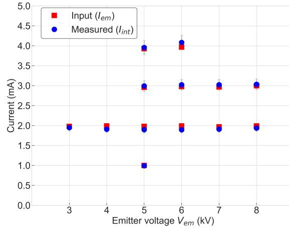
Figure 6.2: Ion current measured ( I_{i_{int}} ) with FC configuration 50.A1.7.P - F.A1.3 for different thruster (LU-C) operation points. The probe is operated with the collector set to -30 V and the repeller to -60 V. The input current ( I_{em} ) is plotted for reference.
