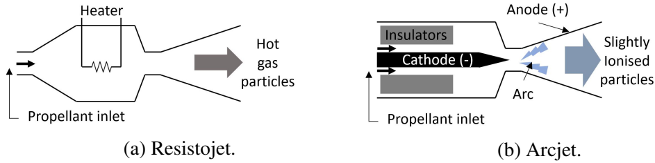
Figure 1.3: Schematic of the working principle of two electro-thermal electric propulsion systems.
